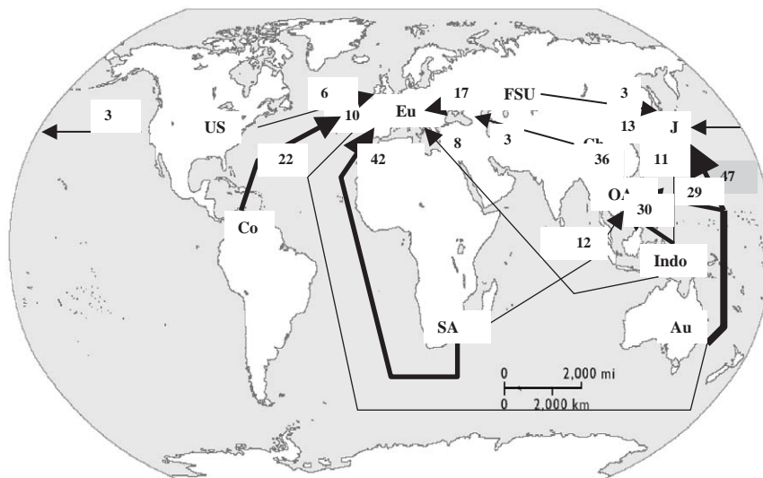
Fig. 3. World steam coal trade routes 2000 (Mt). Source: Own construction based on IEA (2001).
