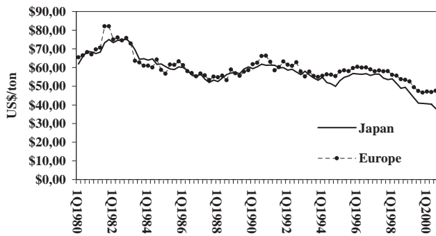
Fig. 2. Import prices for coking coal. Source: IEA (quarterly).
